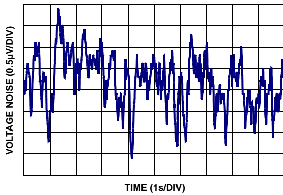
FIGURE 15. EL8170 0.1Hz TO 10Hz INPUT VOLTAGE NOISE (GAIN = 100)
