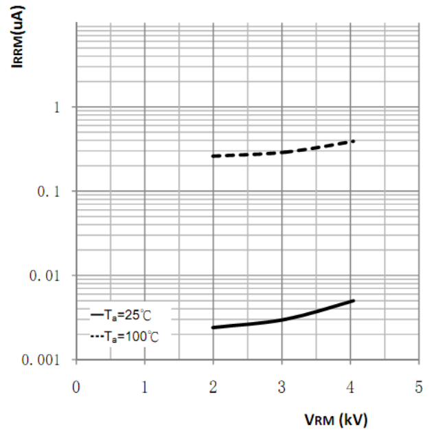
Reverse Characteristics
