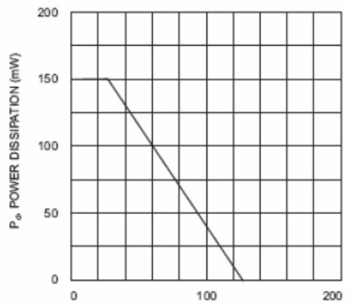
Fig. 4 Power Derating Curve, Total Package
