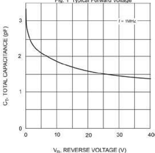
Fig. 3 Typical Capacitance
